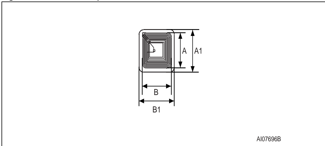
Figure 53. A4 antenna specification
