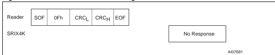
Figure 59. COMPLETION frame exchange between Reader and SRIX4K
