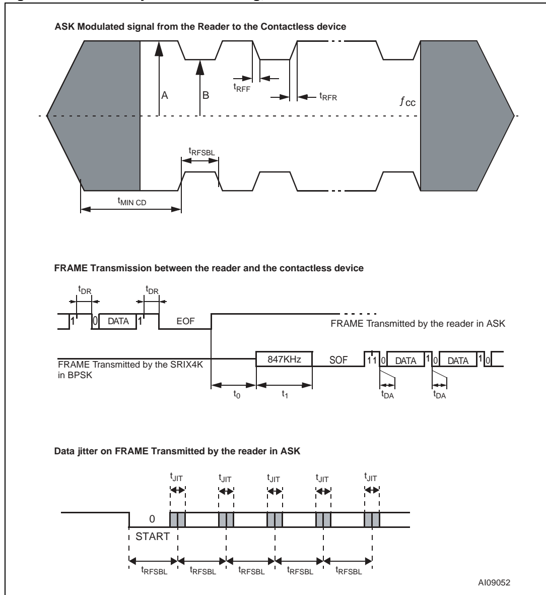
Figure 51. SRIX4K synchronous timing, transmit and receive
