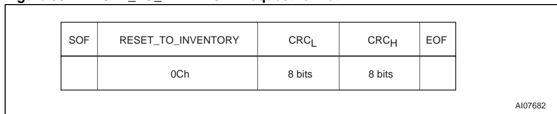
Figure 38. RESET_TO_INVENTORY request format
