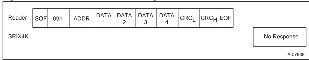
Figure 46. WRITE_BLOCK frame exchange between Reader and SRIX4K
