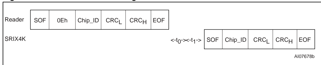
Figure 34. SELECT frame exchange between Reader and SRIX4K
