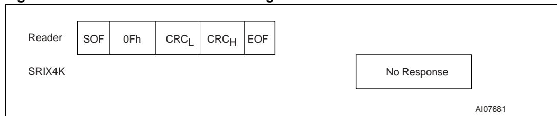
Figure 37. COMPLETION frame exchange between Reader and SRIX4K
