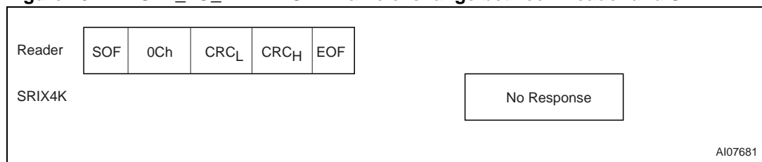
Figure 40. RESET_TO_INVENTORY frame exchange between Reader and SRIX4K
