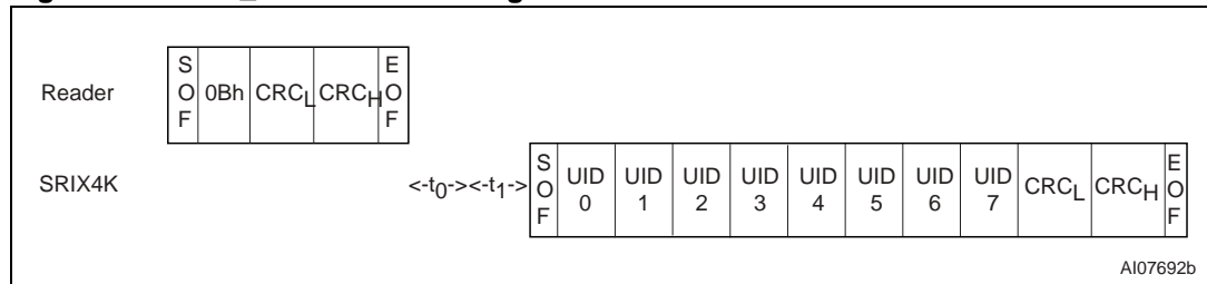
Figure 50. GET_UID frame exchange between Reader and SRIX4K
