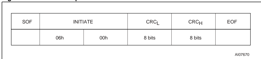
Figure 23. INITIATE request format
