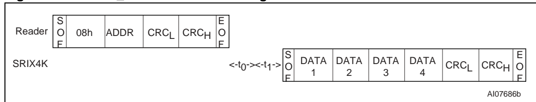
Figure 43. READ_BLOCK frame exchange between Reader and SRIX4K
