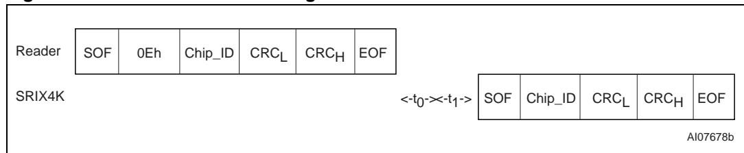
Figure 58. SELECT frame exchange between Reader and SRIX4K
