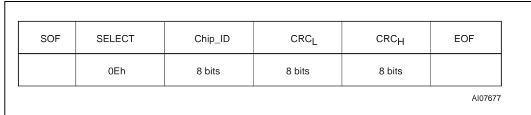
Figure 32. SELECT request format
