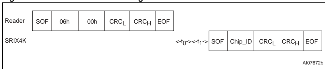
Figure 25. INITIATE Frame Exchange Between Reader and SRIX4K
