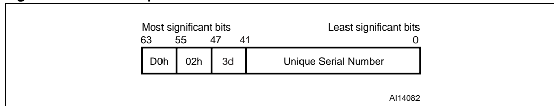
Figure 49. 64-bit unique identifier of the SRIX4K
