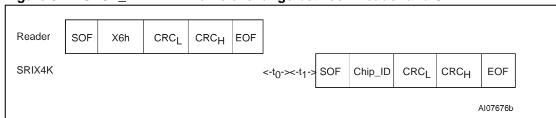
Figure 31. SLOT_MARKER frame exchange between Reader and SRIX4K
