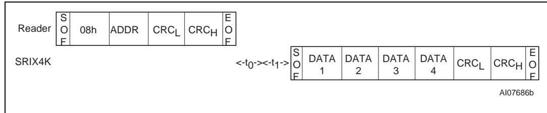
Figure 61. READ_BLOCK frame exchange between Reader and SRIX4K
