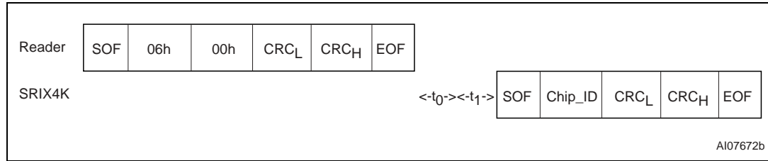
Figure 56. PCALL16 frame exchange between Reader and SRIX4K
