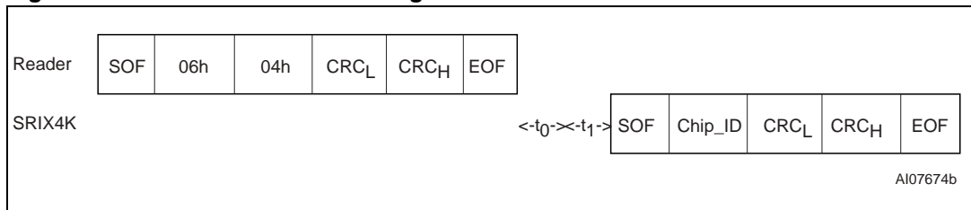
Figure 28. PCALL16 frame exchange between Reader and SRIX4K
