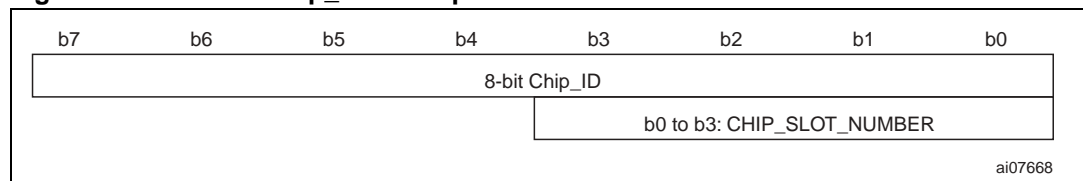
Figure 20. SRIX4K Chip_ID description
