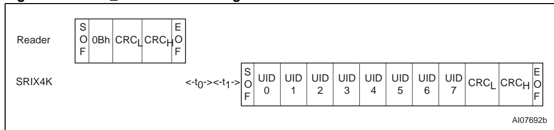
Figure 63. GET_UID frame exchange between Reader and SRIX4K
